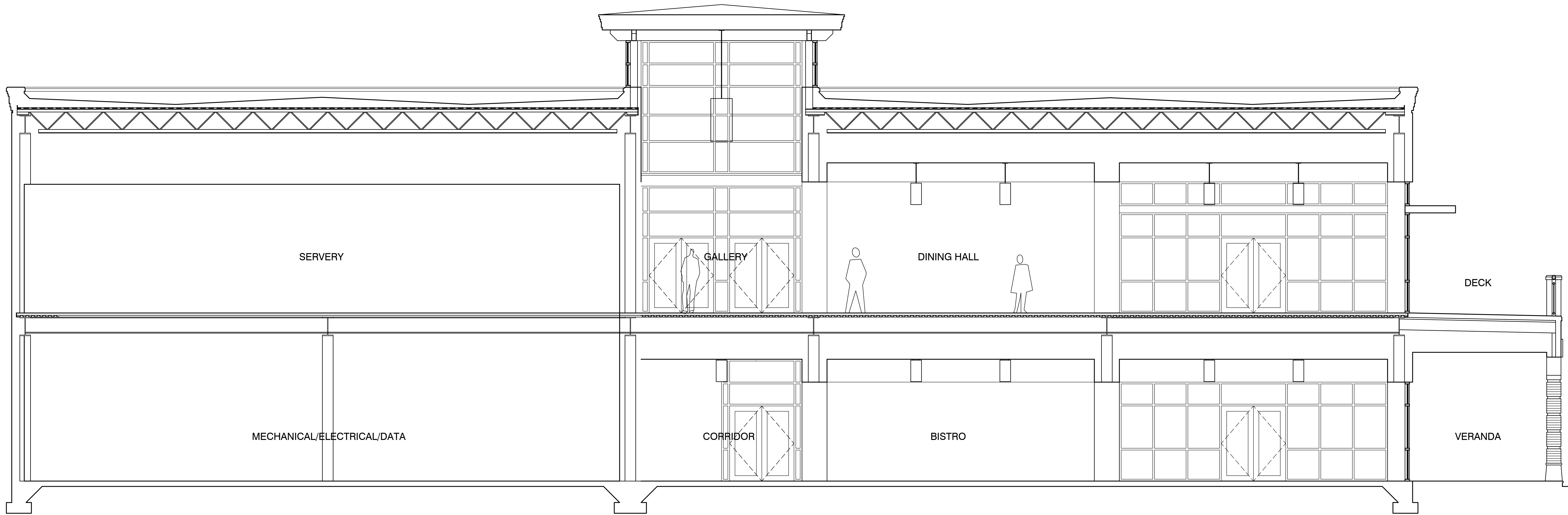
B BUILDING SECTION @ DINING HALL A1.5 1/4" = 1'-0"
