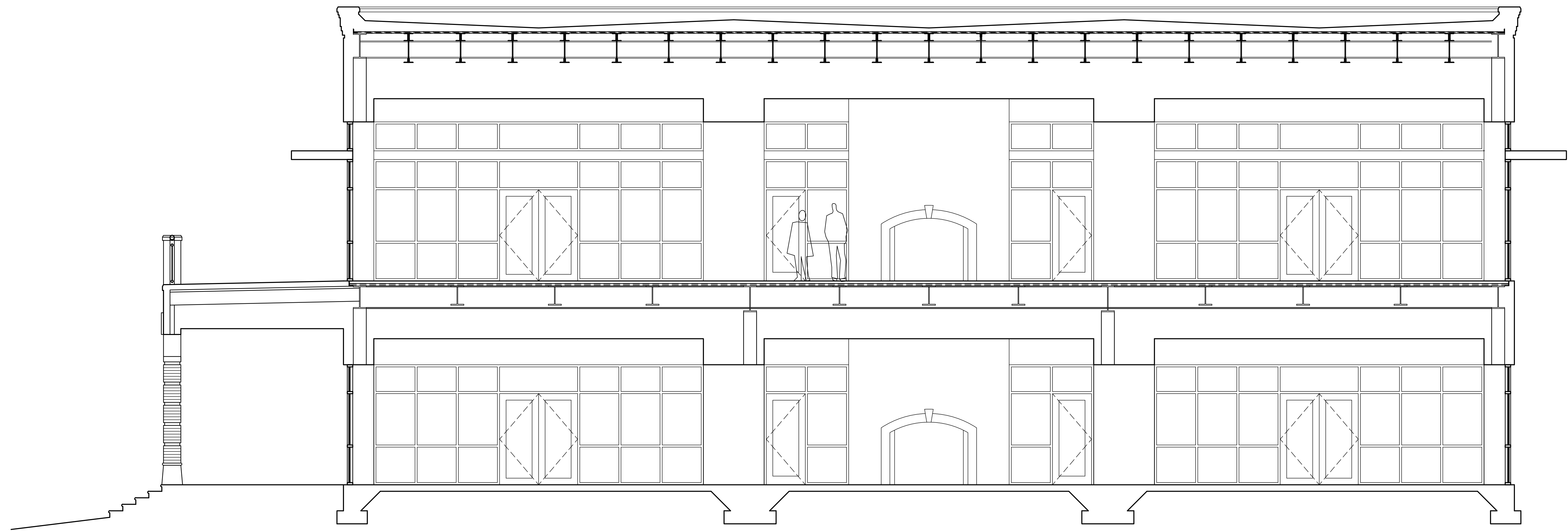
A BUILDING SECTION @ DINING HALL A1.5 1/4" = 1'-0"
